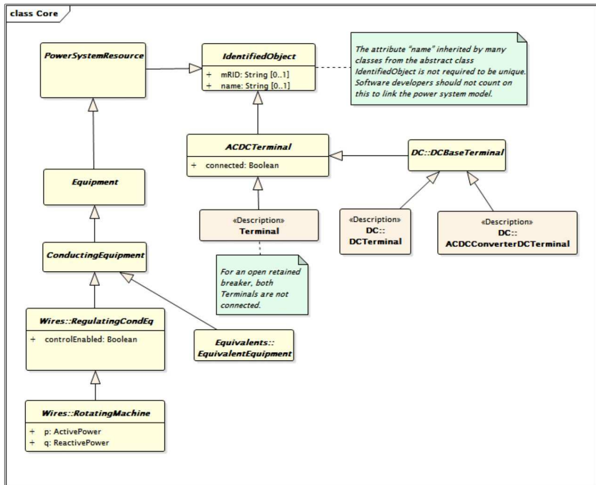
Figure 29 – diagram Core
