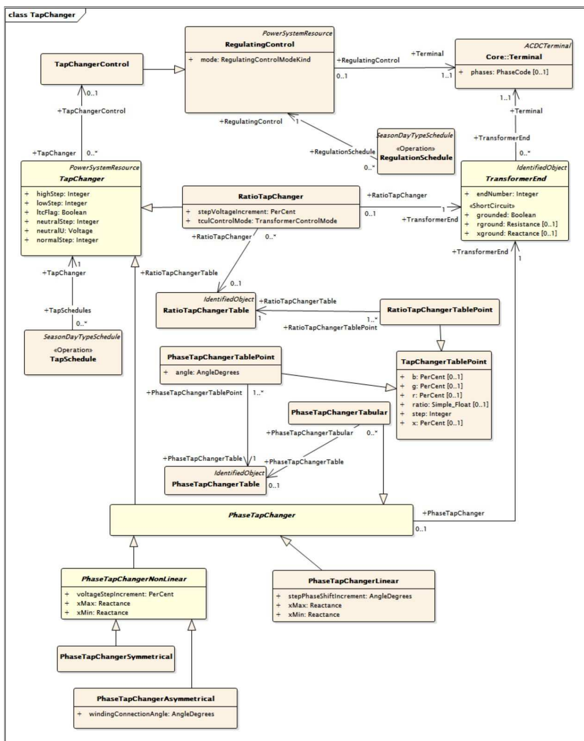
Figure 21 – diagram TapChanger
