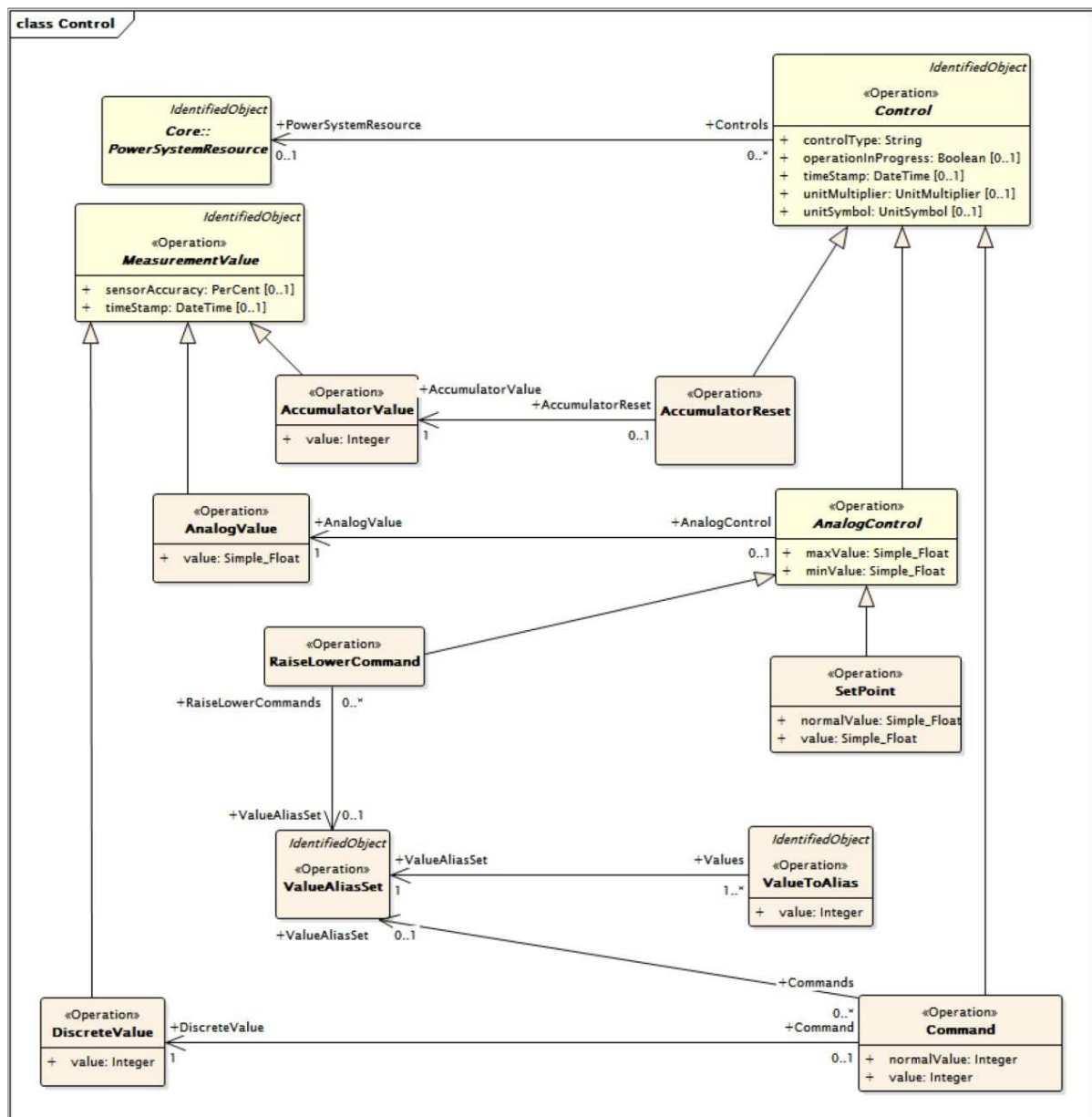
Figure 9 – diagram Control
