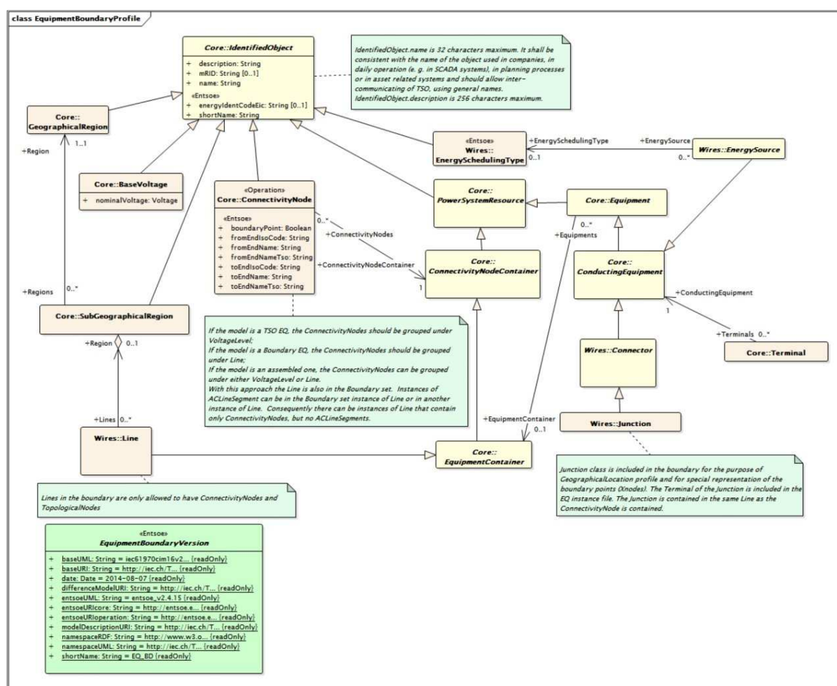
Figure 1 – diagram EquipmentBoundaryProfile
