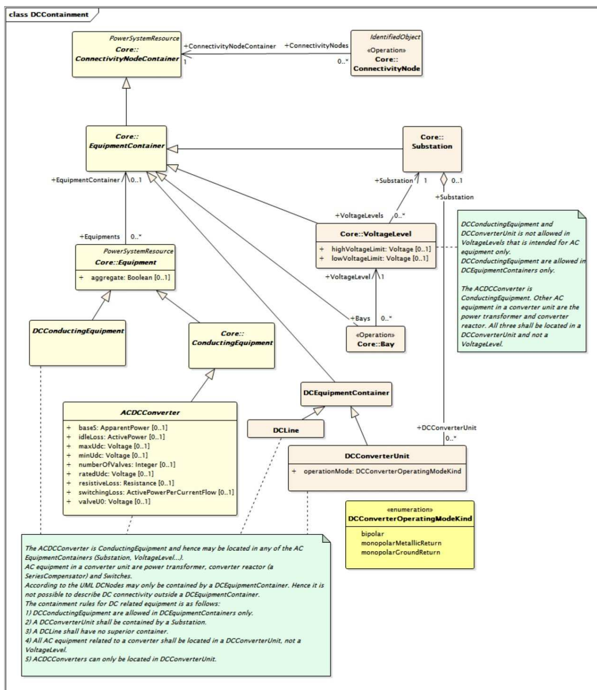
Figure 5 – diagram DCContainment
