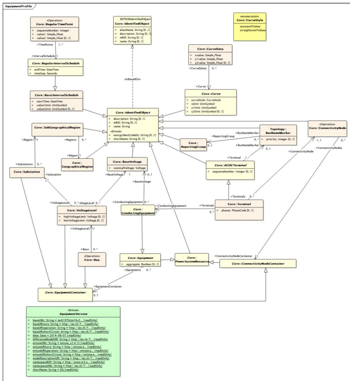
Figure 3 – diagram EquipmentProfile
