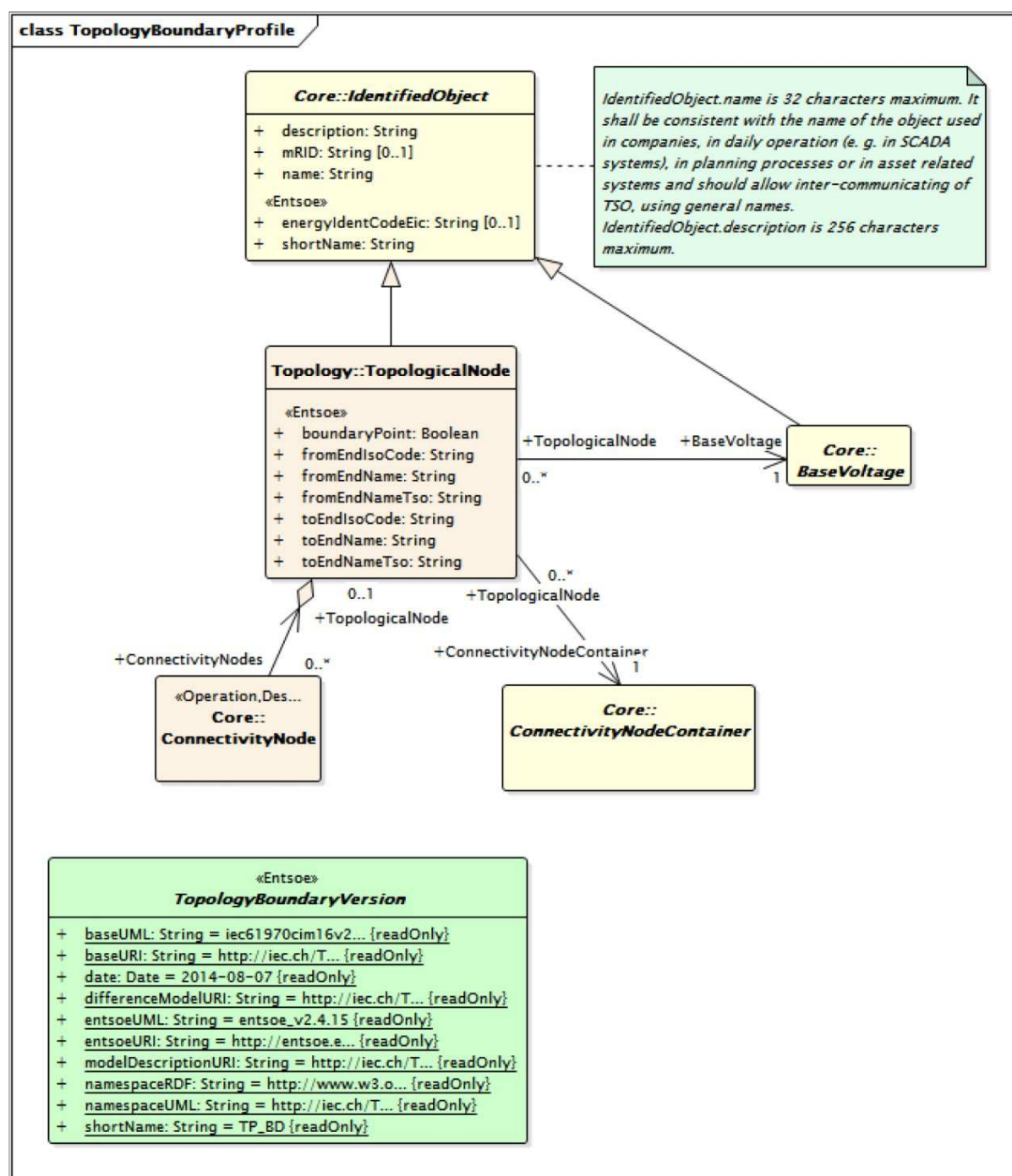
Figure 2 – diagram TopologyBoundaryProfile
