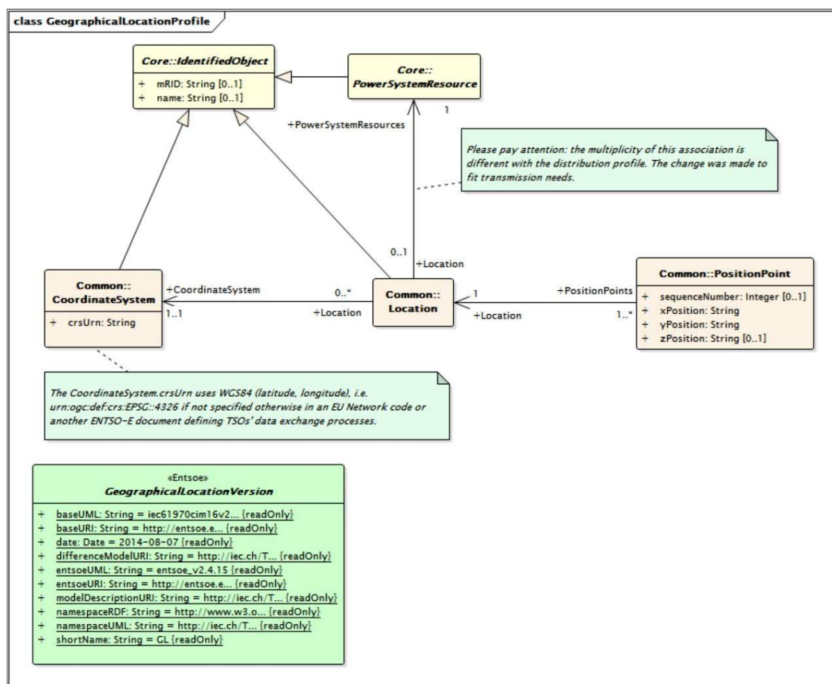
Figure 41 – diagram GeographicalLocationProfile
