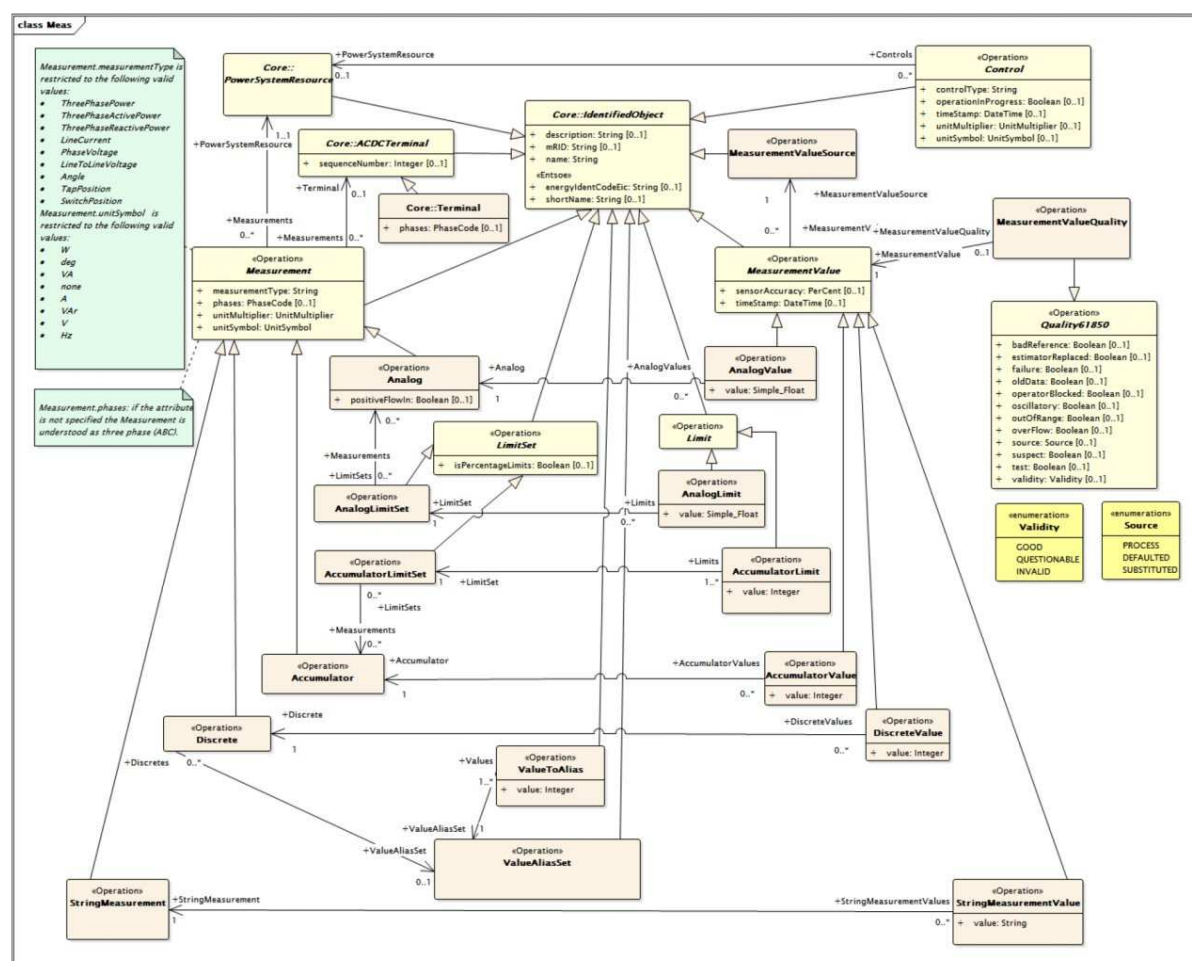
Figure 10 – diagram Meas
