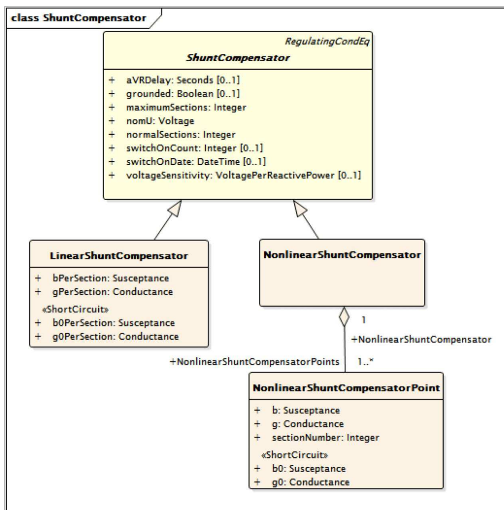
Figure 18 – diagram ShuntCompensator
