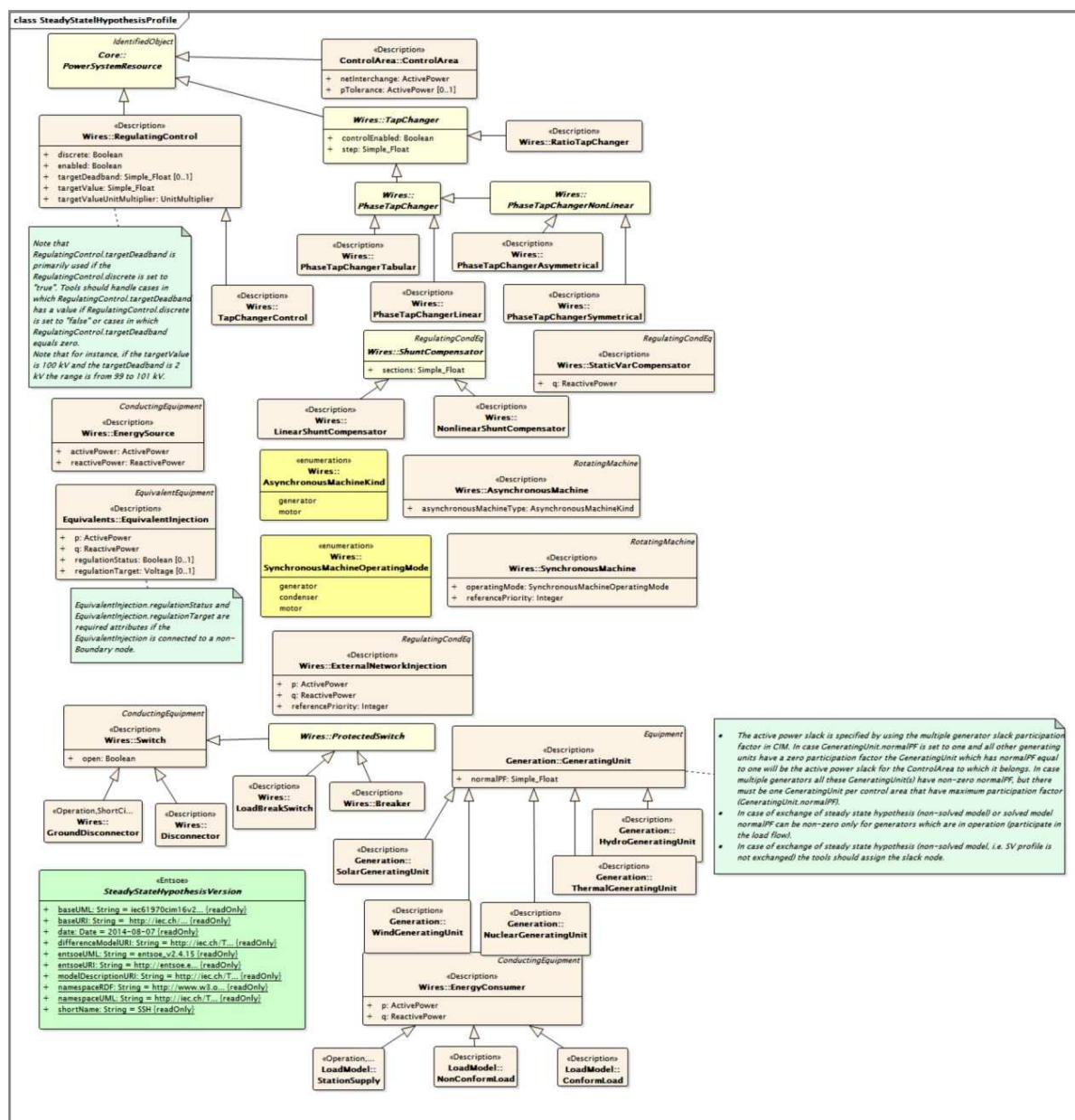
Figure 28 – diagram SteadyStateHypothesisProfile
