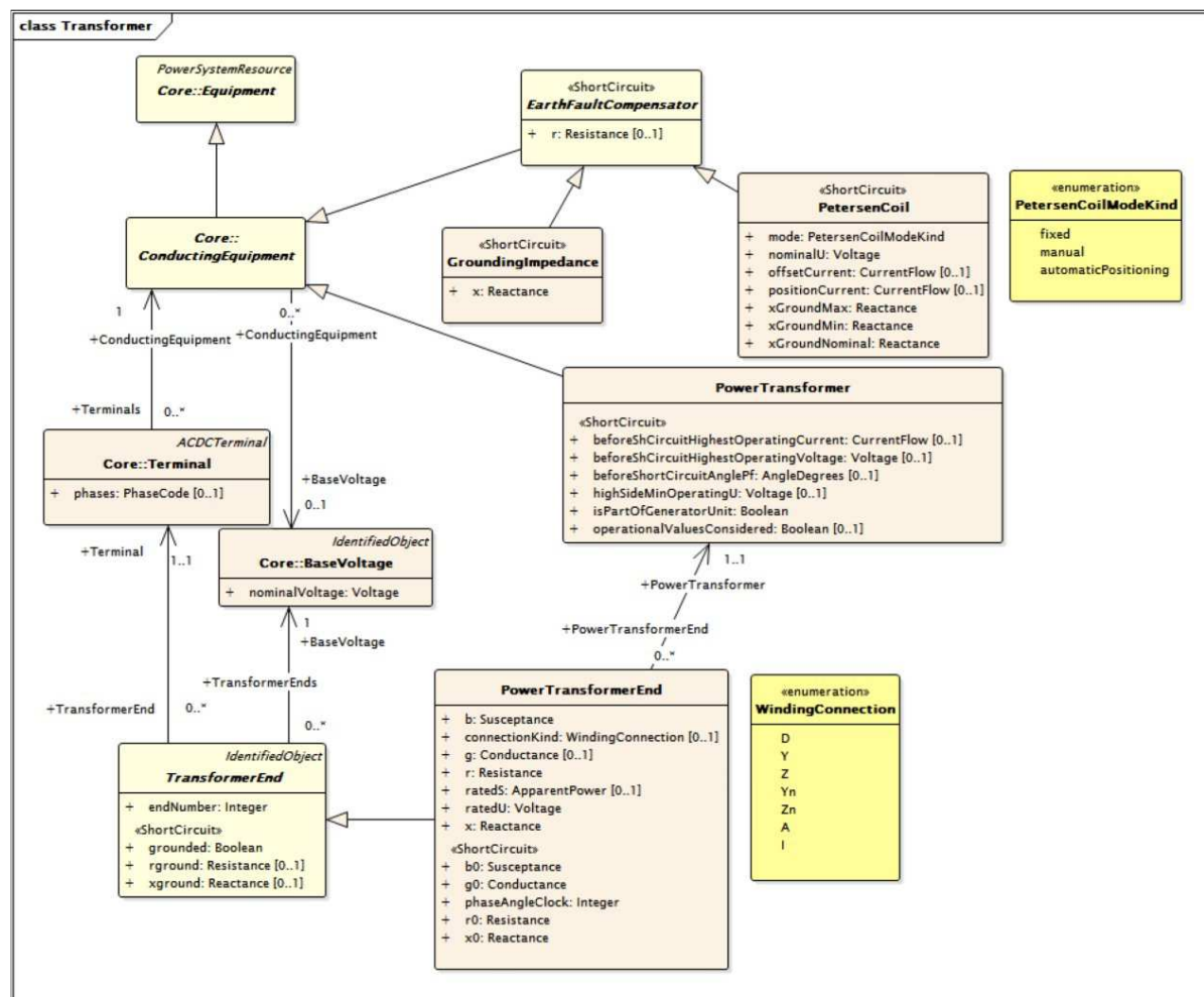
Figure 22 – diagram Transformer
