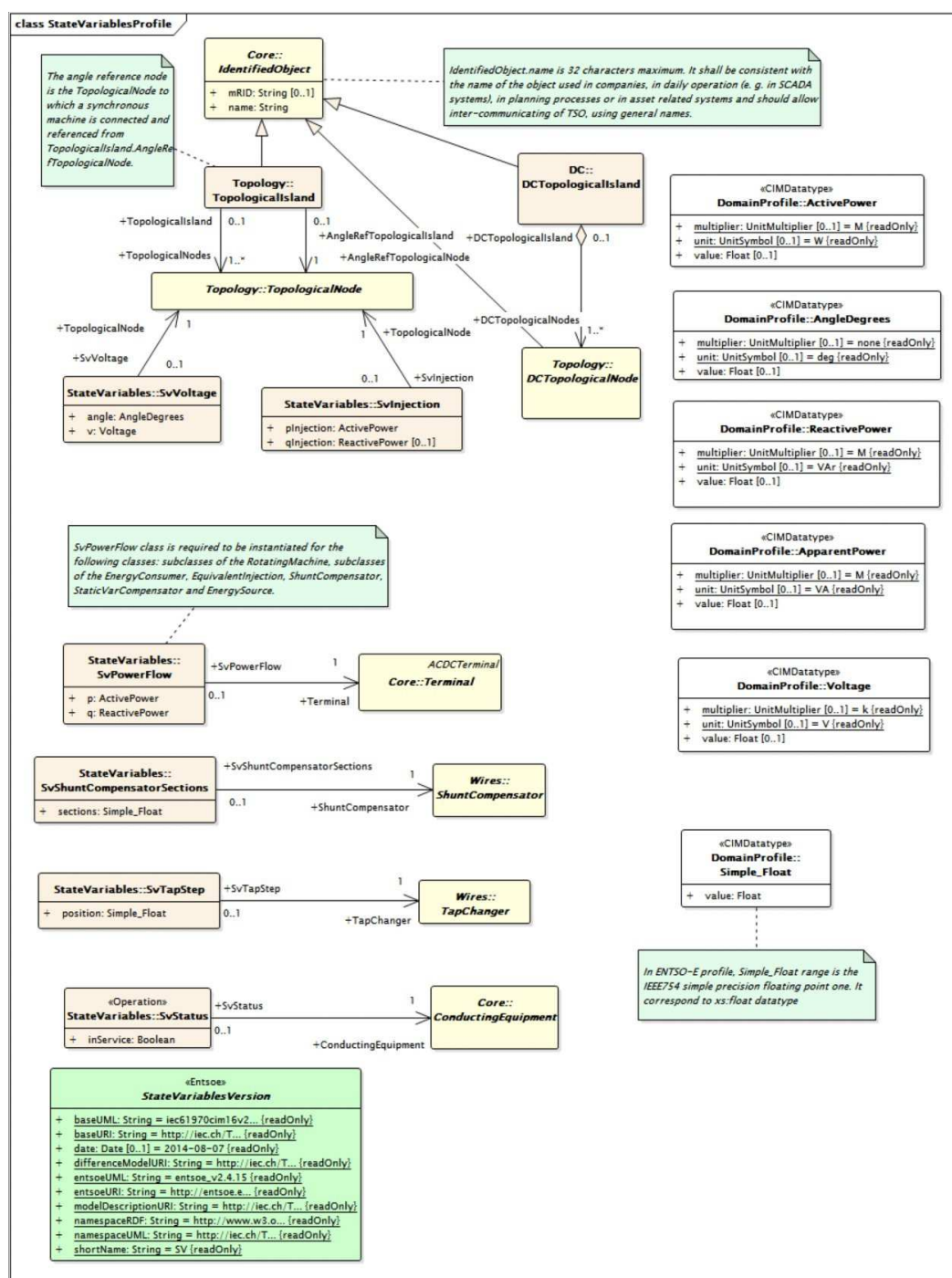
Figure 35 – diagram StateVariablesProfile
