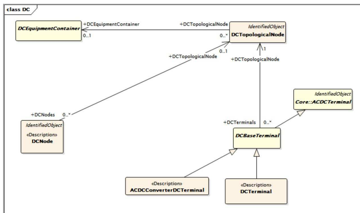
Figure 34 – diagram DC
