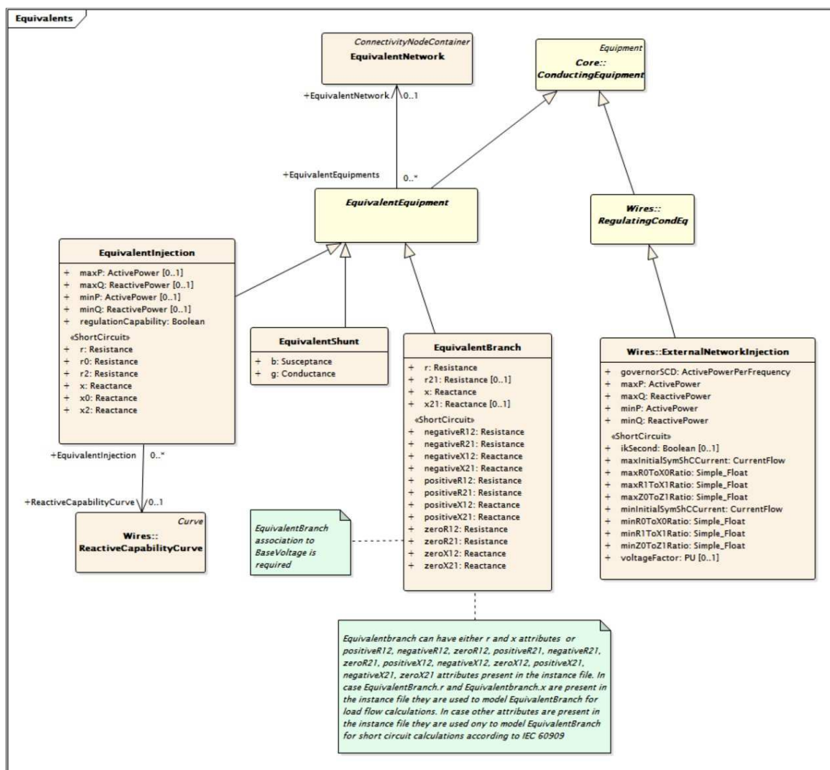
Figure 25 – diagram Equivalents
