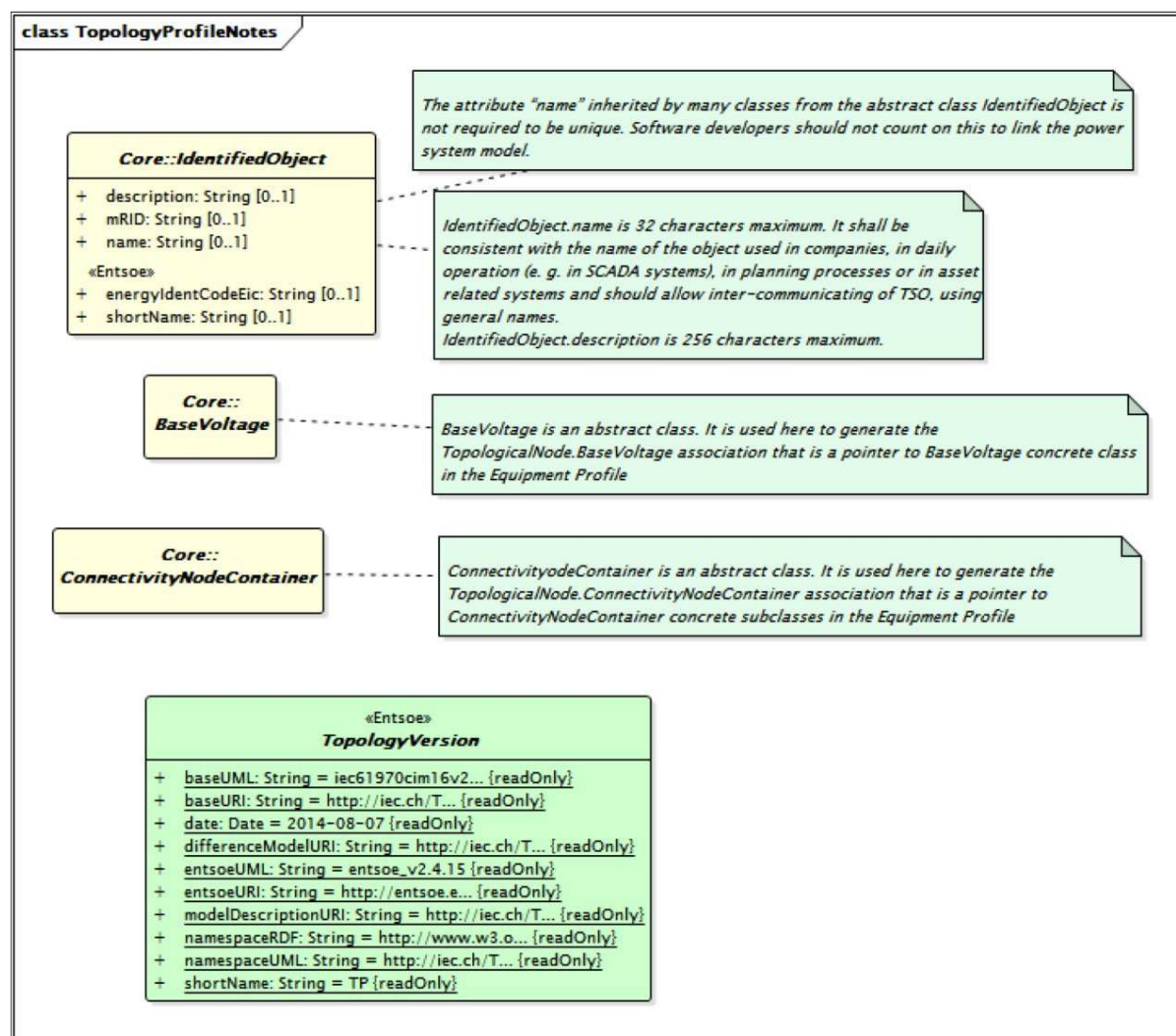
Figure 31 – diagram TopologyProfileNotes
