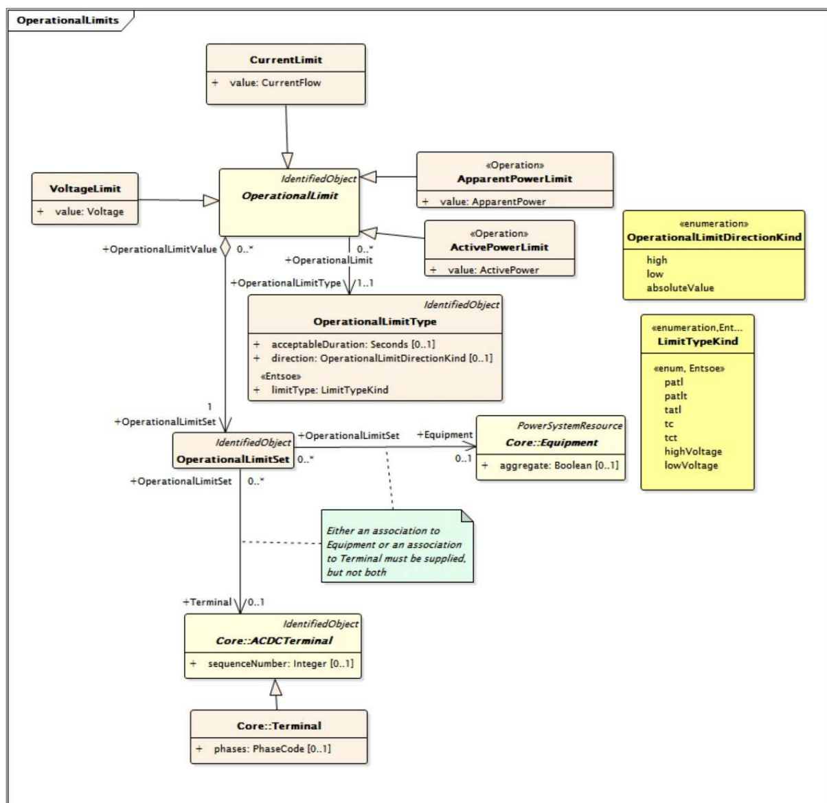
Figure 16 – diagram OperationalLimits
