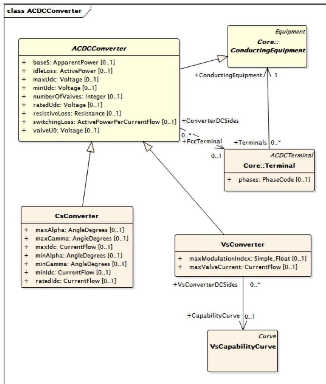
Figure 4 – diagram ACDCCConverter
