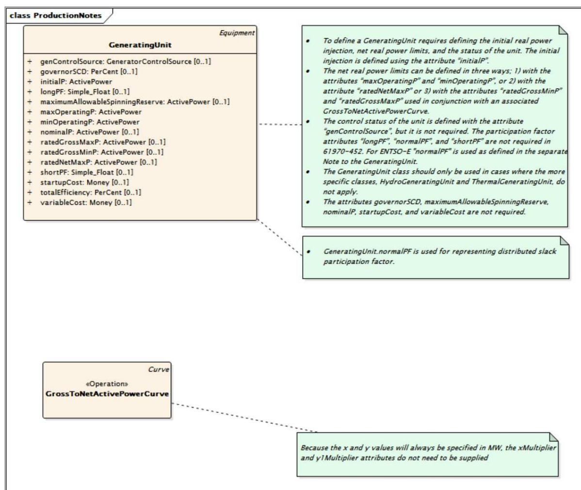
Figure 13 – diagram ProductionNotes
