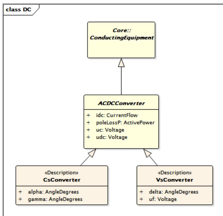
Figure 37 – diagram DC
