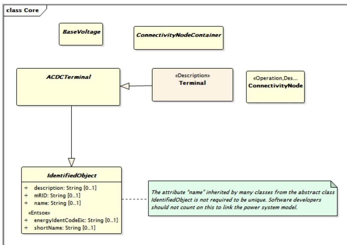
Figure 33 – diagram Core
